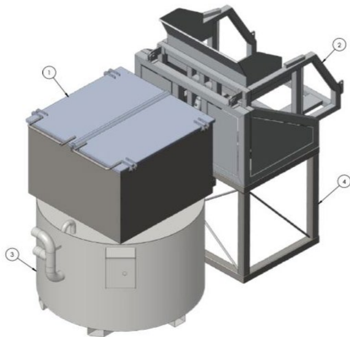
Figure 3.1: Primary silage unit from Stensvik in Norway. Secondary tanks for storing the prepared silage would also be required.
