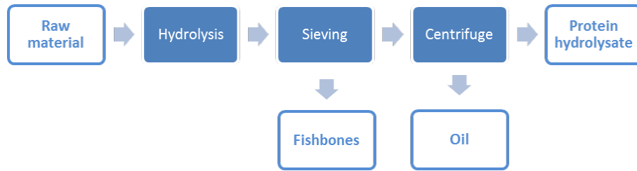
Figure 1.13: Simplified schema of protein hydrolysate process
